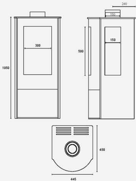
F500 Slim Freestanding
