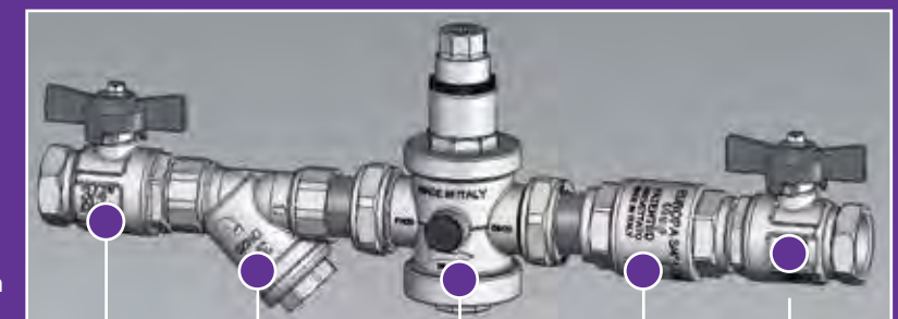
Ball Valve Y Strainer Pressure Reducing Valve Non Return Valve Ball Valve
