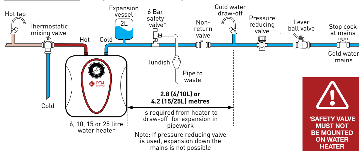
Fig. 3: For inlet water pressure ABOVE 4.1 BAR, a pressure reducing valve is required. Where REQUIRED DISTANCE FOR PIPEWORK EXPANSION IS NOT AVAILABLE - 2.8M FOR 6/10L & 4.2M FOR 15/25L, an expansion vessel is required.
