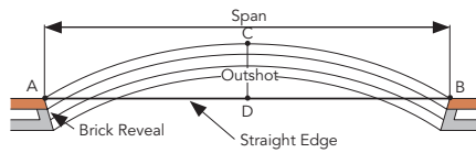
Bow Lintel with Non Projecting Reveals
