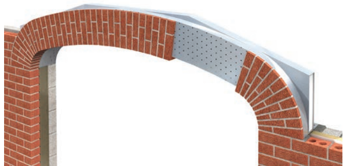
KEYSTONE'S APEX ARCH BRICK SLIP FEATURE LINTEL
